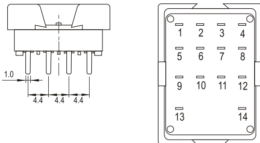
Terminal Arrangement (Bottom View)
